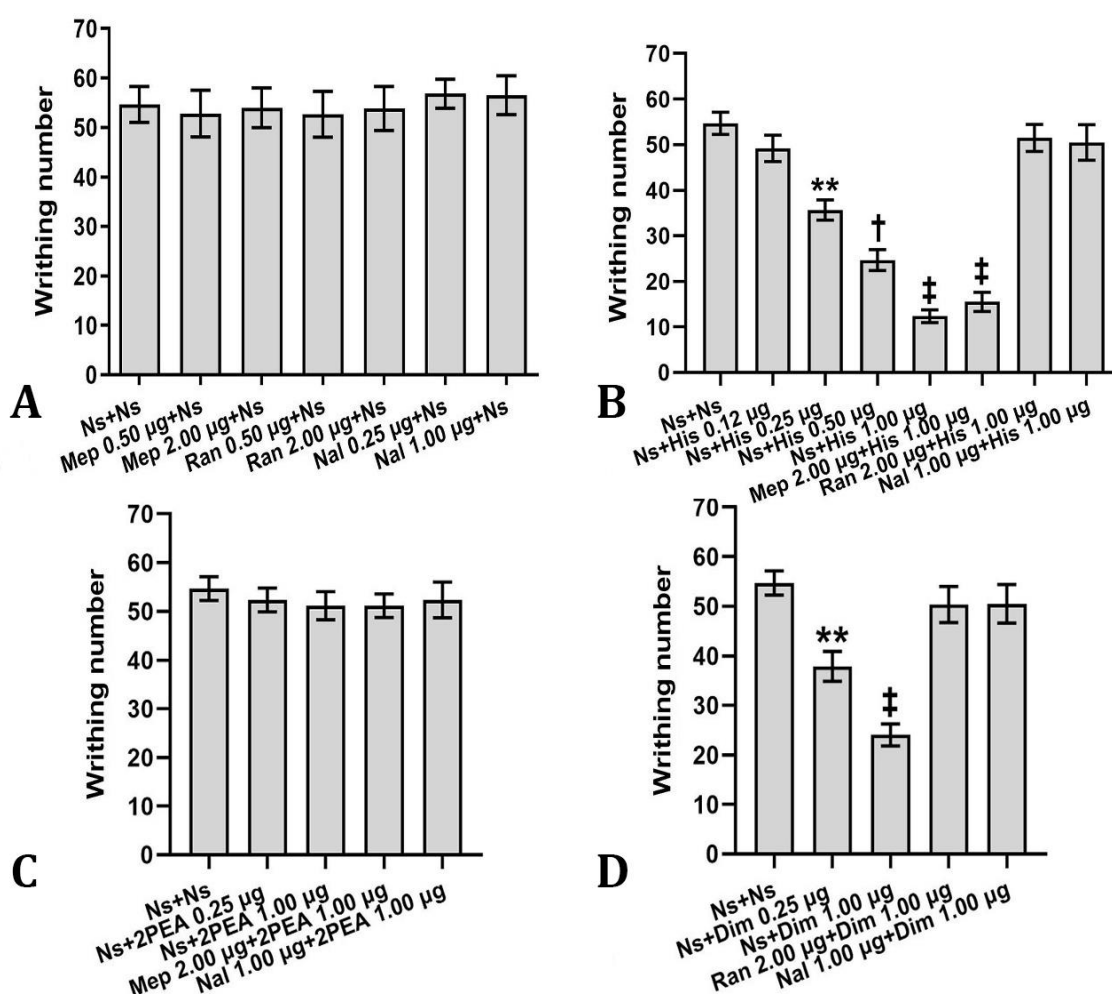
Fig. 3. Nociceptive response (writhing number over 60 min) induced by intraperitoneal injection of acetic acid after intra-fastigial nucleus (FN) microinjection of A) mepyramine (Mep), ranitidine (Ran) and naloxone (Nal), B) histamine (His), mepyramine plus histamine, ranitidine plus histamine and naloxone plus histamine, C) 2-pyridylethylamine (2-PEA), mepyramine plus 2-PEA and naloxone plus 2-PEA and D) dimaprit (Dim), ranitidine plus dimaprit and naloxone plus dimaprit. In all the double microinjections into the FN, time intervals of 4.00 and 2.00 minutes were observed before induction of visceral pain. All drugs were administered as \mu\text{g} per 240 \text{g}^{-1} . Ns: normal saline. Values from each group are the mean \pm SEM ( n = 6 ). ** p < 0.01 , † p < 0.001 and ‡ p < 0.0001 compared to Ns+Ns, respectively.
