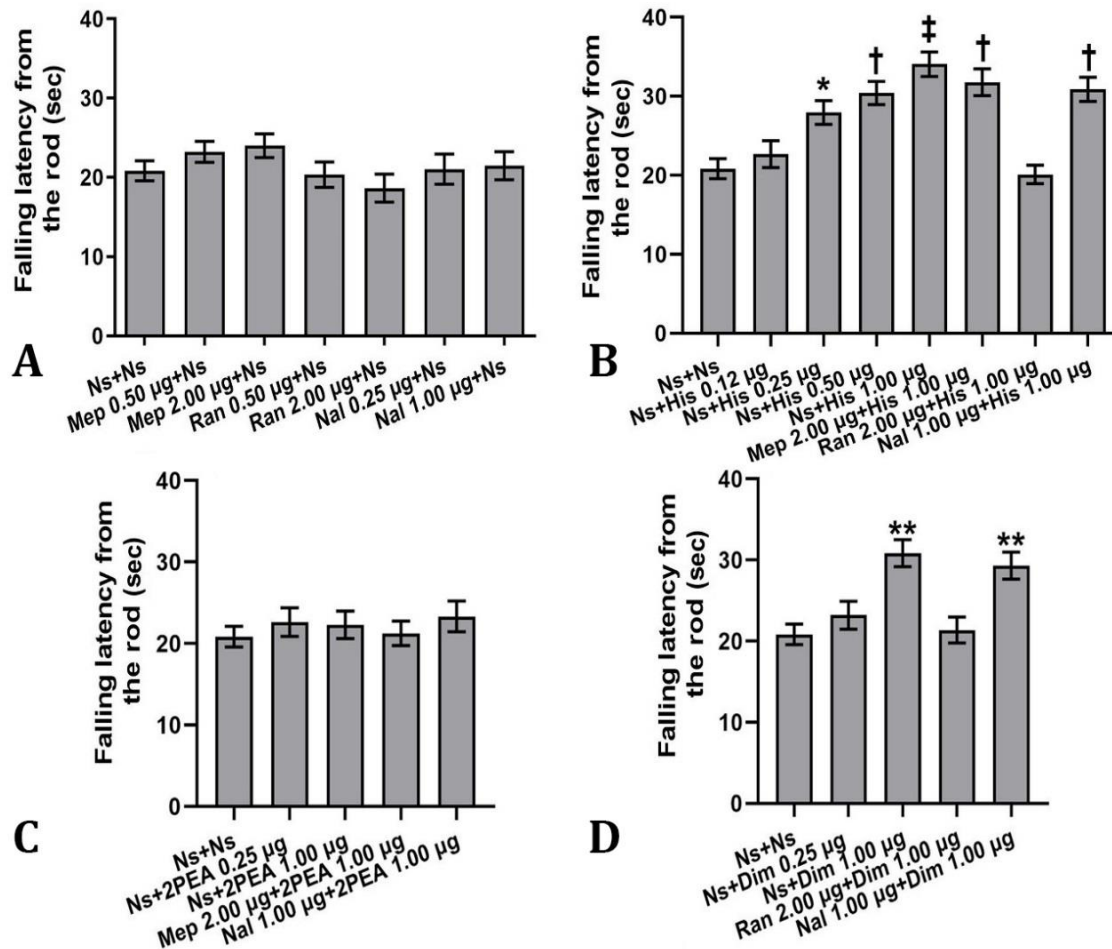
Fig. 4. Fall latency from the rod after intra-fastigial nucleus (FN) microinjection of of A ) mepyramine (Mep), ranitidine (Ran) and naloxone (Nal), B ) histamine (His), mepyramine plus histamine, ranitidine plus histamine and naloxone plus histamine, C ) 2-pyridylethylamine (2-PEA), mepyramine plus 2-PEA and naloxone plus 2-PEA and D ) dimaprit (Dim), ranitidine plus dimaprit and naloxone plus dimaprit. In all the double microinjections into the FN, time intervals of 4.00 and 2.00 minutes were observed before induction of visceral pain. All drugs were administered as µg per 240 g. Ns: normal saline. Values from each group are the mean \pm SEM (n = 6). ** p < 0.01 , † p < 0.001 and ‡ p < 0.0001 compared to Ns+Ns, respectively.
