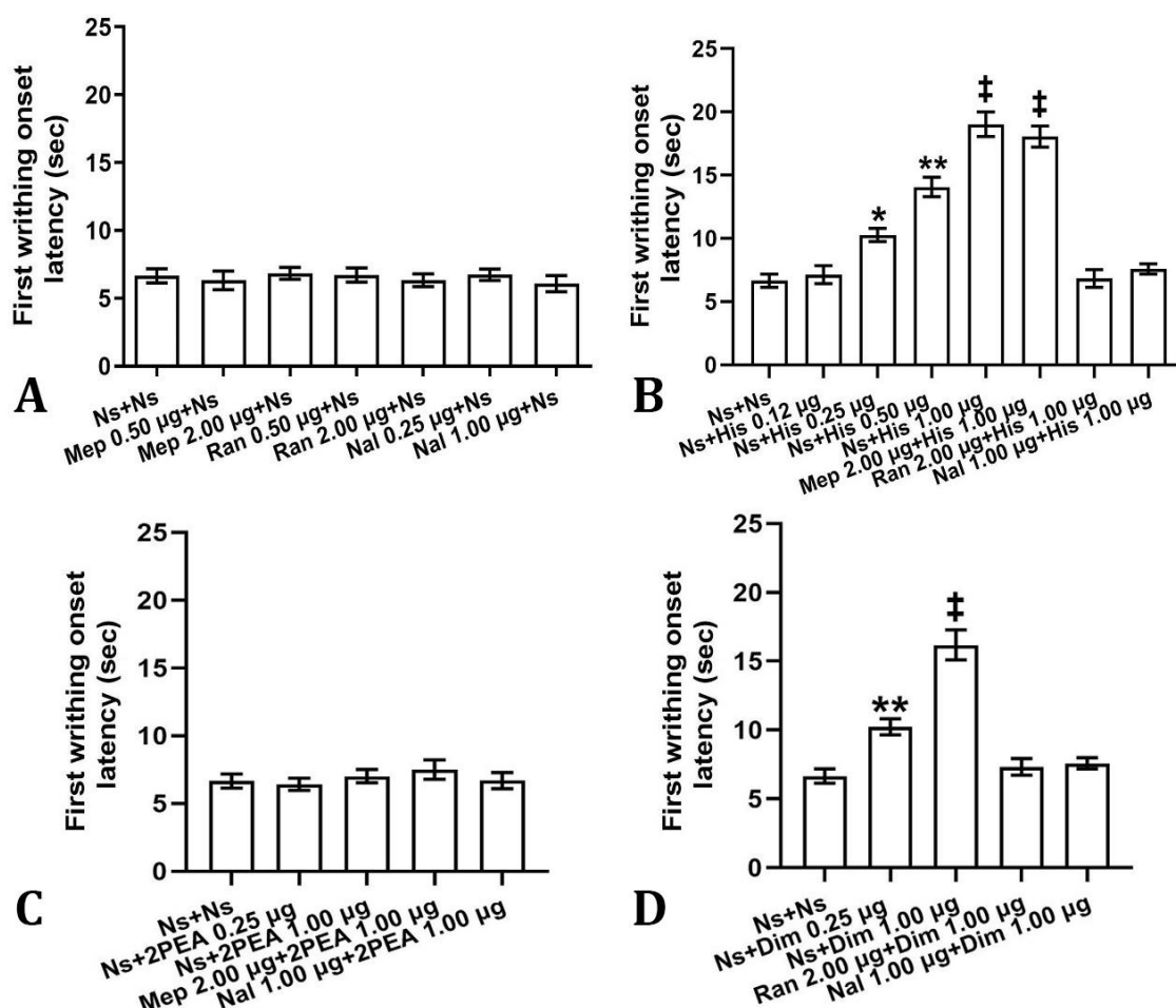
Fig. 2. Nociceptive response (first writhing latency time) induced by intraperitoneal injection of acetic acid after intra-fastigial nucleus (FN) microinjection of A ) mepyramine (Mep), ranitidine (Ran) and naloxone (Nal), B ) histamine (His), mepyramine plus histamine, ranitidine plus histamine and naloxone plus histamine, C ) 2-pyridylethylamine (2-PEA), mepyramine plus 2-PEA and naloxone plus 2-PEA and D ) dimaprit (Dim), ranitidine plus dimaprit and naloxone plus dimaprit. In all the double microinjections into the FN, time intervals of 4.00 and 2.00 minutes were observed before induction of visceral pain. All drugs were administered as \mu\text{g} per 240 \text{g}^{-1} . Ns: normal saline. Values from each group are the mean \pm SEM ( n = 6 ). * p < 0.05 , ** p < 0.01 , † p < 0.001 and ‡ p < 0.0001 compared to Ns+Ns, respectively.
